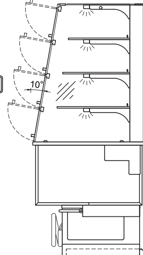
Glass Enclosure slanted DROP-IN
