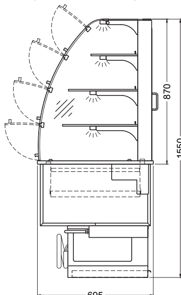
Glass Enclosure curved DROP-IN
