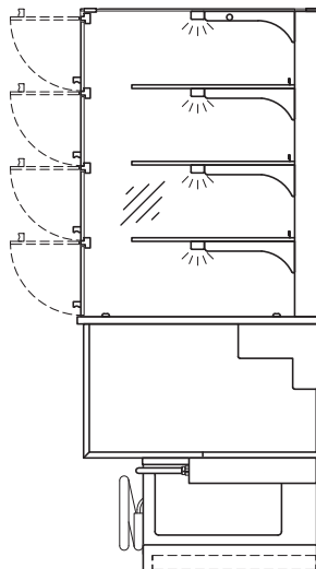
Glass Enclosure squared DROP-IN
