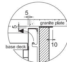
Detail A: built under granite
